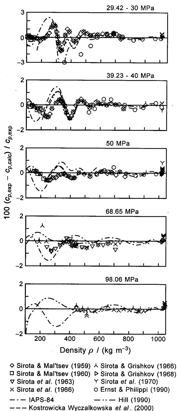
FIG. 7.36. Percentage deviations between experimental data of the isobaric heat capacity c_p in the extended critical region and values calculated from IAPWS-95, Eq. (6.4). Values calculated from IAPWS-84, the equation of Hill (1990), and the crossover equation of Kostrowicka Wyczalkowska et al. (2000) are plotted for comparison; the crossover equation is only shown within its range of validity. The two lowest diagrams and the density range of all diagrams extend beyond the extended critical region.
