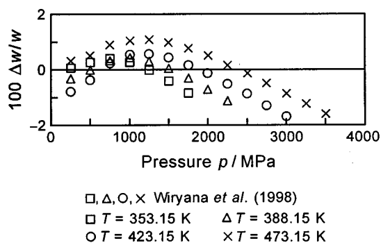
FIG. 7.25. Percentage deviations 100\Delta w/w = 100(w_{\text{exp}} - w_{\text{calc}})/w_{\text{exp}} between the experimental data of the speed of sound w of Wiriyana et al. (1998) for temperatures from 353.15 to 473.15 K and values calculated with IAPWS-95, Eq. (6.4). For the pressures above 1000 MPa, IAPWS-95 was extrapolated.
